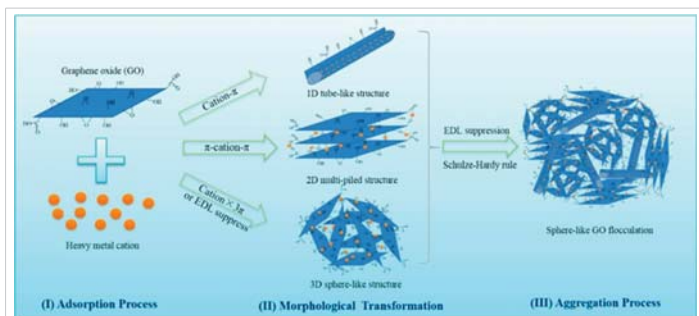
Figure 11: From Environ. Sci. Technol. 2016, 50, 20, 11066-11075 Proposed interactions of heavy metal cations with GO nanosheets in 3 steps: (1) adsorption of heavy metal onto GO nano-sheets; (2) formation of 1D-, 2D-, and 3D-like structures; and (3) aggregation of sphere-like flocculation
