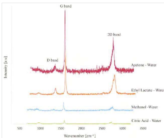
Figure 10: Raman spectra RS of graphene exfoliated via different solvent systems. An increase in the D peak is observed as the lowest R-value of a particular system decreases. This suggests better exfoliation due to the presence of more edges as more layers are exfoliated from bulk- material. It can be seen in Figure that the D band which is associated with edge defects increases gradually when graphene was exfoliated in solvent-water systems that have to decrease Ra- values. This is characteristic of better exfoliation due to the formation of the new edges which leads to a more pronounced edge effect reflected by the increase in the D- peak.
